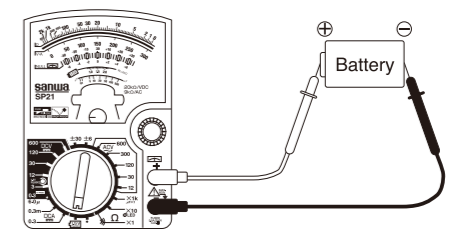
Battery voltage
